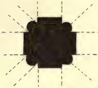
Fig. 332.—Rivolta d'Adda. Church of Santa Maria e San Sigismondo. Section of one of the large piers (XIth Century).
